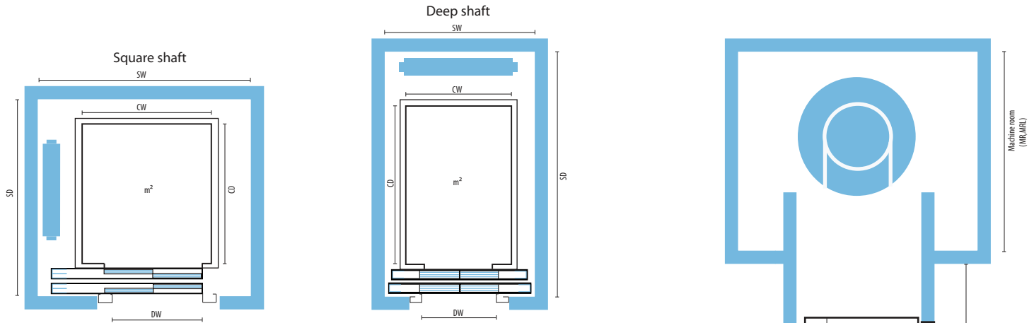
AV120 shaft plan table
